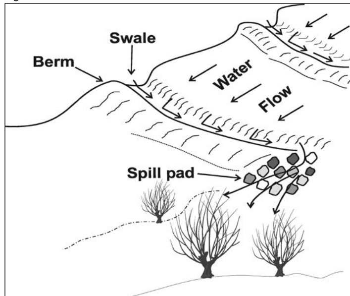
Figure 2. Diversion drains.
