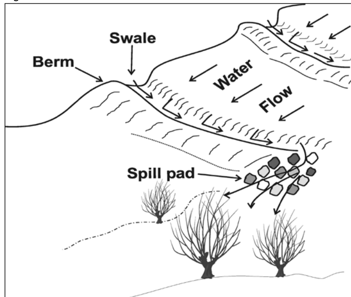
Figure 2. Diversion drains.
